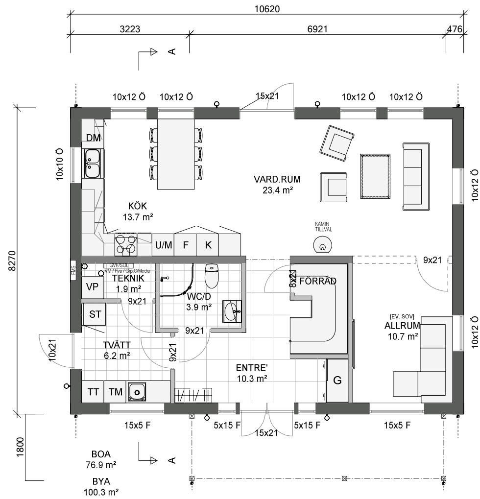
BOTTENPLAN
